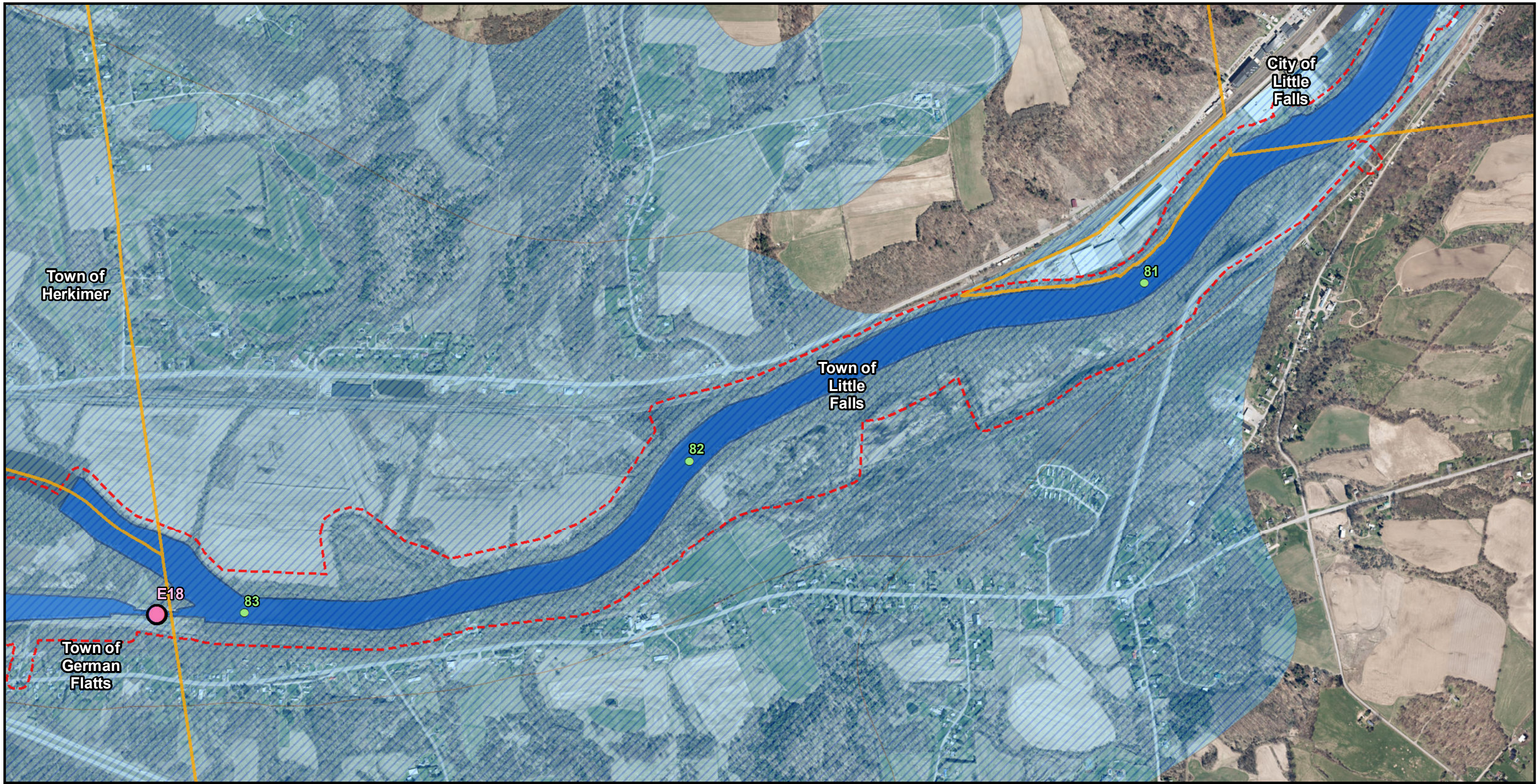
Figure 40F: Aquifers
